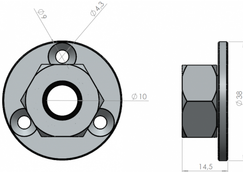
Outline Drawing
