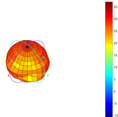
Total_3D_Side View 1_1.57542GHz
