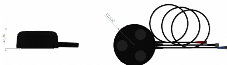
48033-000 - Magnetic Mounting - Outline Drawing
