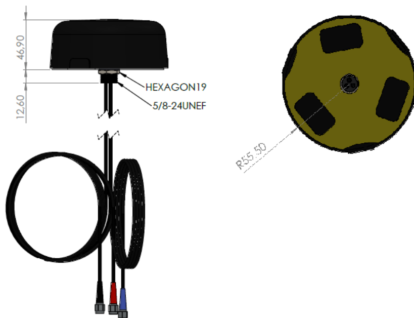
48013-000 - Through Hole Mounting - Outline Drawing
