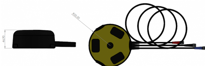
48023-000 - Adhesive Mounting - Outline Drawing
