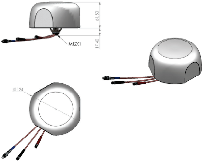
Outline Drawing
