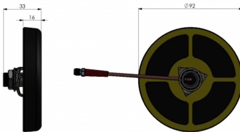
outline drawing
