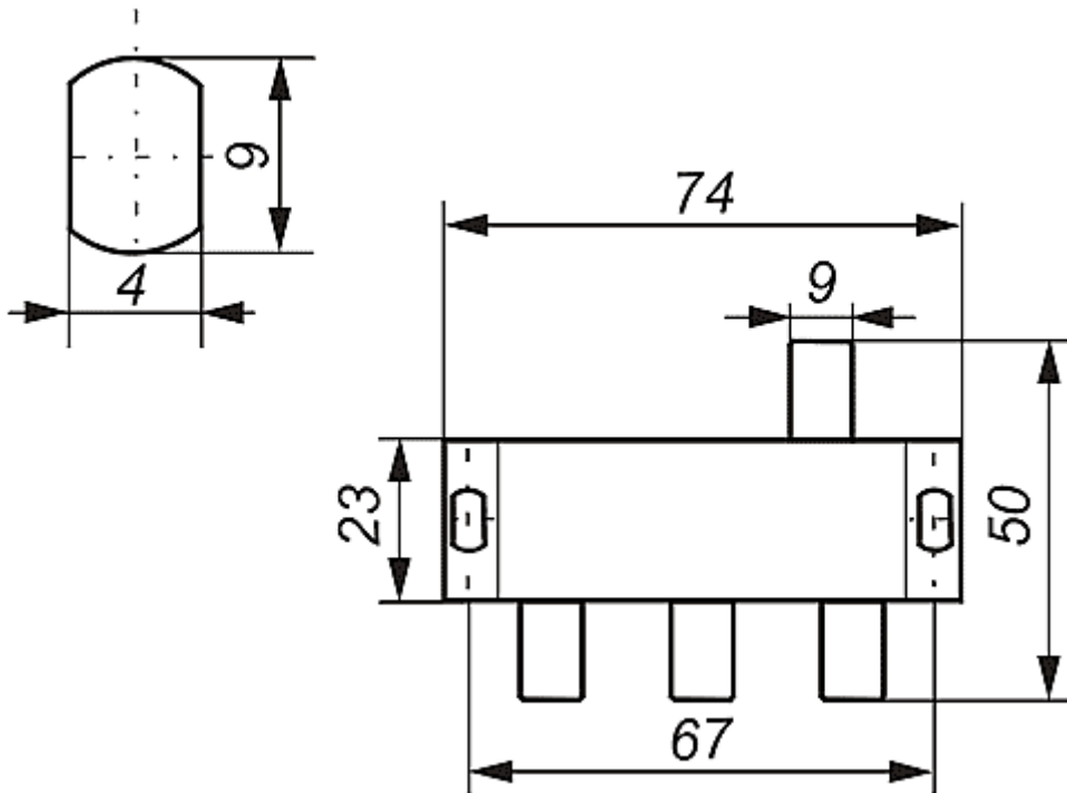
Dimensions [mm]
