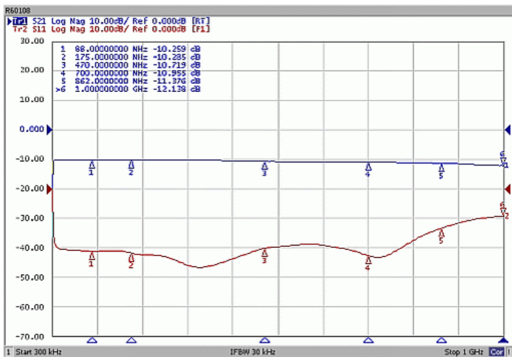
Loss and return loss diagram
