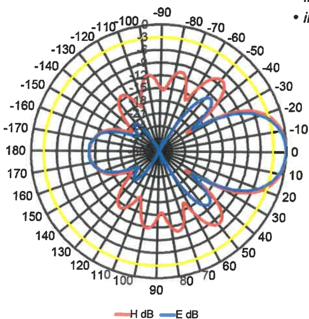
RADIATION PATTERN
