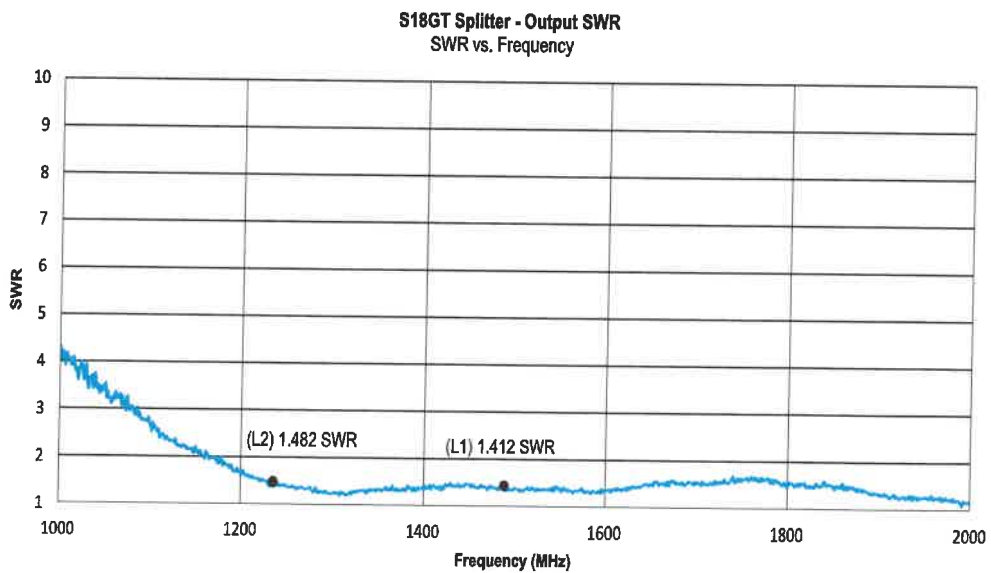
Figure 2-2. Output SWR (10dB)
