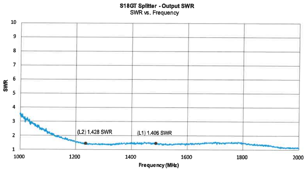
Figure 2-4. Output SWR (0dB)
