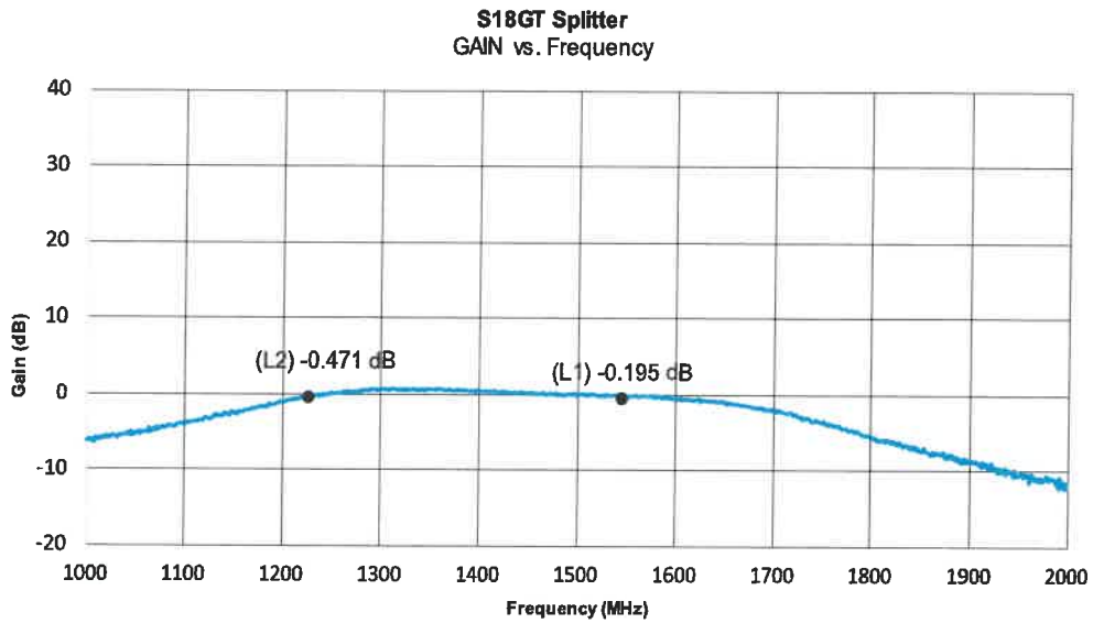
Figure 2-3. Frequency Response (0dB)
