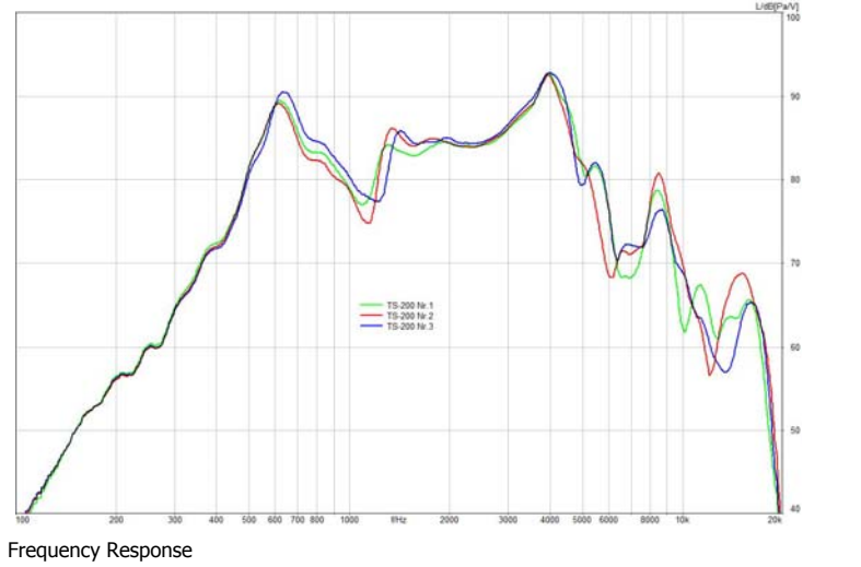
b. 3x SPL Frequency Response @1W/1m
