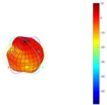
Total_3D_Front View_2.7GHz
